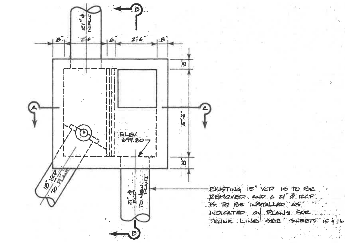
CONTROL CHAMBER NO. 1 PLAN VIEW NOT TO SCALE
