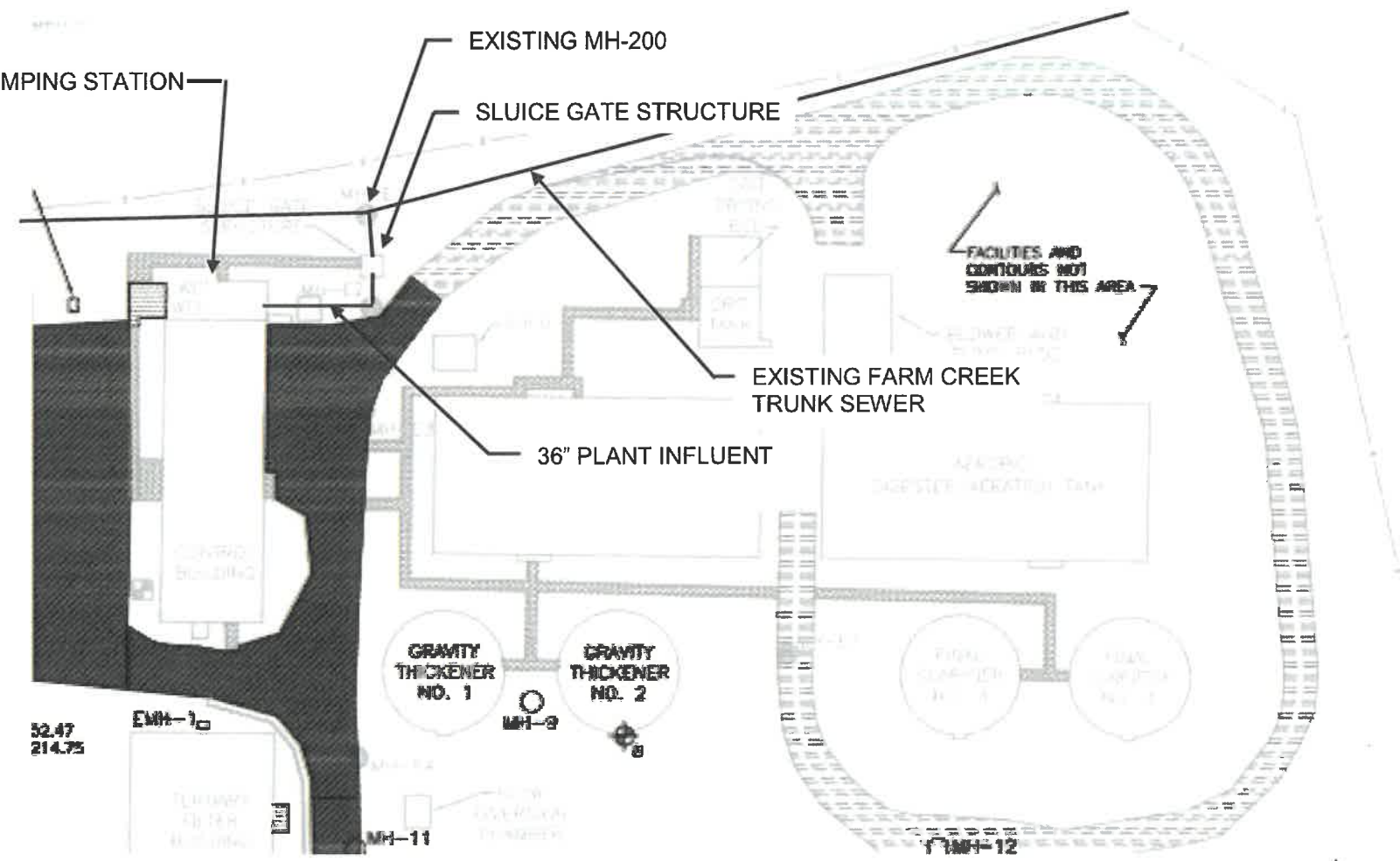
STP-2 SITE PLAN NOT TO SCALE
