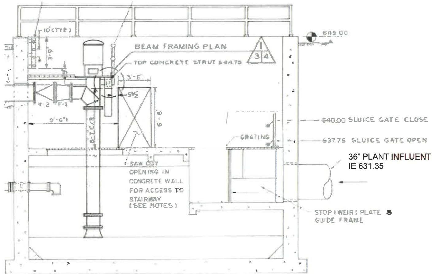
INFLUENT PUMPING STATION A-A NOT TO SCALE
