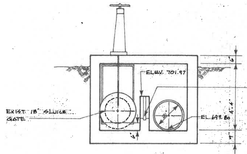
CONTROL CHAMBER NO. 1 A-A NOT TO SCALE
