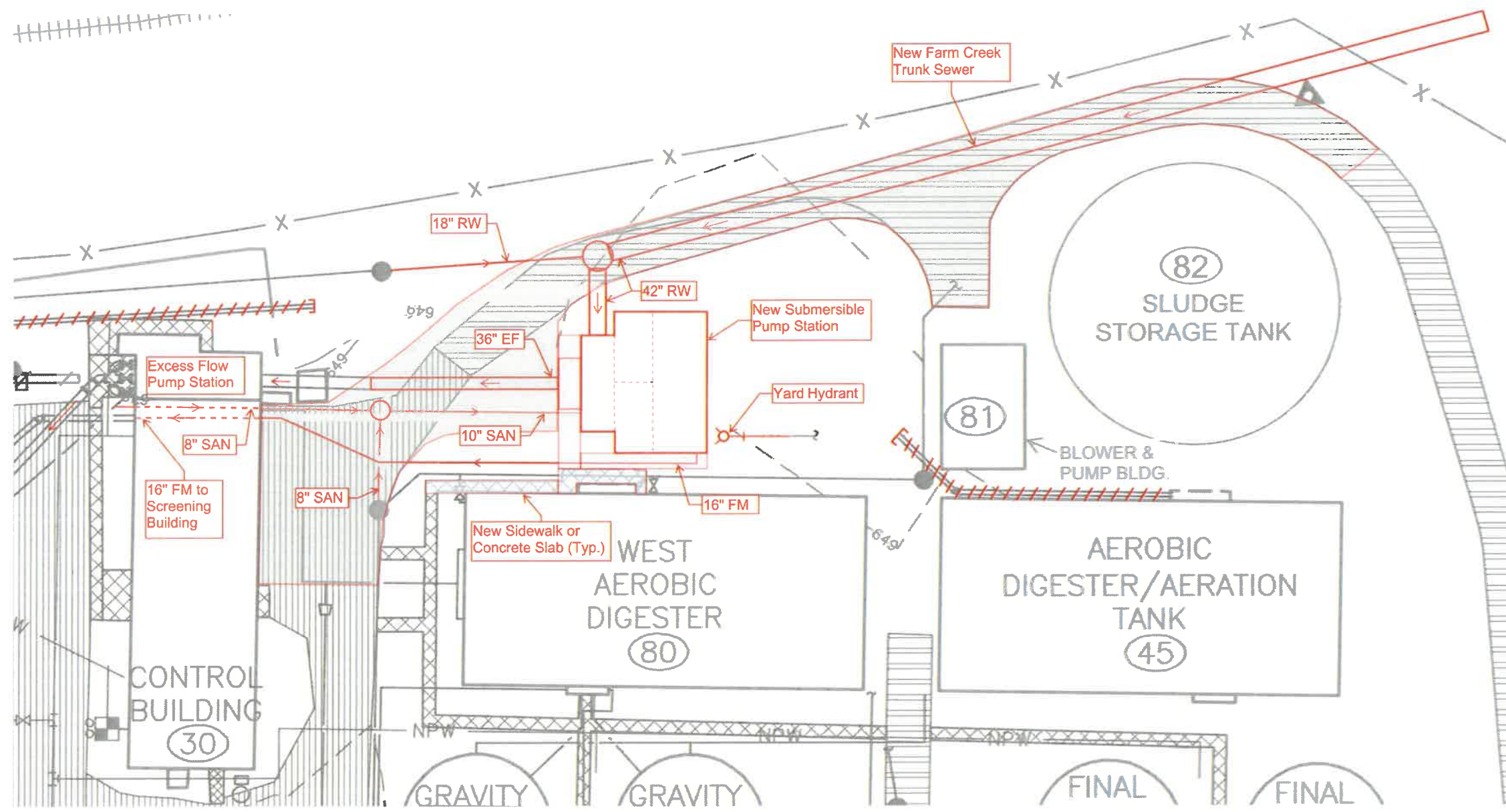
Site Plan (no scale) ↑ North
