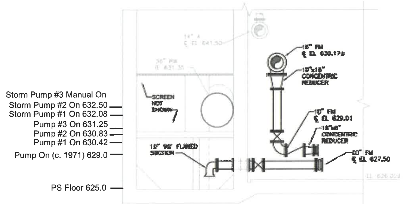
INFLUENT PUMPING STATION B-B NOT TO SCALE
